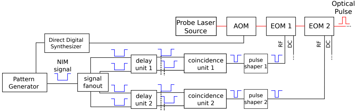
Figure 2.7: Schematic diagram of the optical pulse generation process from a continuous probe laser beam.
