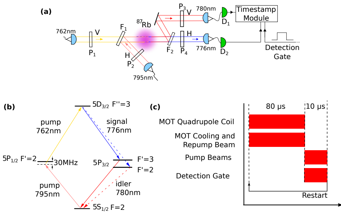
Figure 2.13: (a) Schematic diagram of the experimental setup for FWM in collinear configuration. P 1 and P 3 select the vertical polarisation (V) while P 2 and P 4 select the horizontal polarisation (H). F 1 and F 2 : Interference filters. D 1 and D 2 : Silicon Avalanche Photo-Diode. (b) 87 Rb level transitions in FWM. (c) Experimental sequence for the generation of the correlated photon pair.
