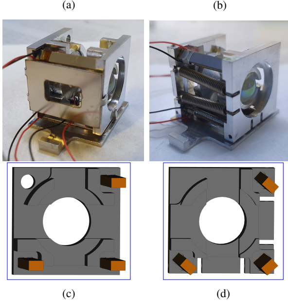
FIG. 3: (a) Structure using a 3 contact point clamp. (b) Structure using springs. (c) Actuator base parallel to the mirror frame. (d) Actuator base rotated by 45^\circ from the mirror frame.
