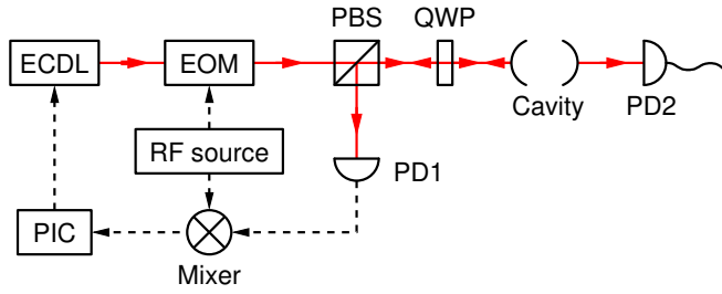
FIG. 5: Schematic of the experimental setup. ECDL: external cavity diode laser; EOM: electro-optical modulator; PIC: proportional proportional integral control; PBS: polarized beamsplitter; QWP: quater quarter waveplate; PD: photodiode.
