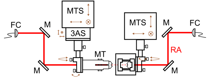
FIG. 4: Alignment setup of the NC cavity. RA: reference axis, FC: fibre-fiber coupler, M: mirror, MT: mechanical tweezer, MTS: manual translation stage, 3AS: three-axis actuator stage.
