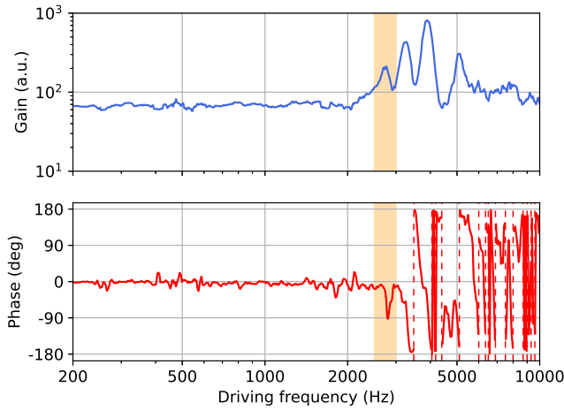
FIG. 7: Cavity response to the stimulus sent to the piezoelectric actuators. Shaded region highlights the first resonance of the cavity, centered at 2750Hz.
