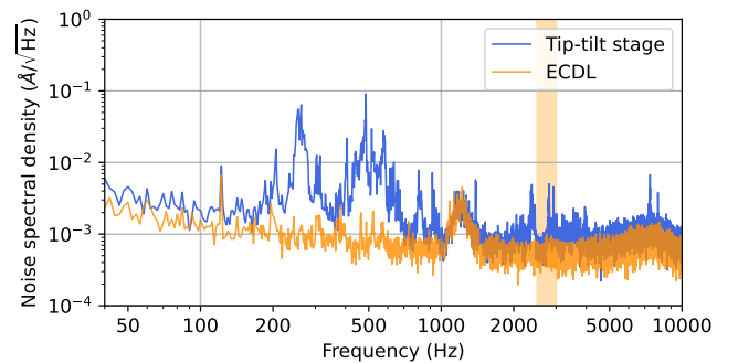
FIG. 6: Noise spectral density of the cavity length over an integration time of 0.5 s. Total The measurement is conducted at a critical distance of d = 1.06(5) \mu\text{m} for the NC cavity. The total displacement noise is 0.36(92) \text{ \AA}_{rms} . The shaded region highlights the first resonance of the cavity, centered at 2750 Hz (see Figure 7).
