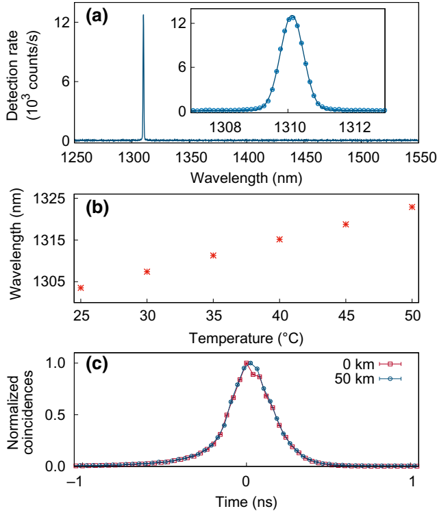
FIG. 2. (a) The spectrum of signal photons from the nondegenerate pair source at a temperature of 33.4\ ^{\circ}\text{C} of the PPKTP crystal shows a single peak around 1310 nm with a nearly Gaussian profile (see fit to the data in the inset). (b) Signal photon wavelength dependence on PPKTP temperature. (c) Time correlation of photon detection events from a pair of APDs, with the signal photon passing through 0 and 50 km of SMF28e+ fiber, respectively. The temporal correlations for the 50 km transmission case are offset and normalized for visual comparison. Both histograms show a nearly indistinguishable distribution with a full width at half maximum around 280 ps.
