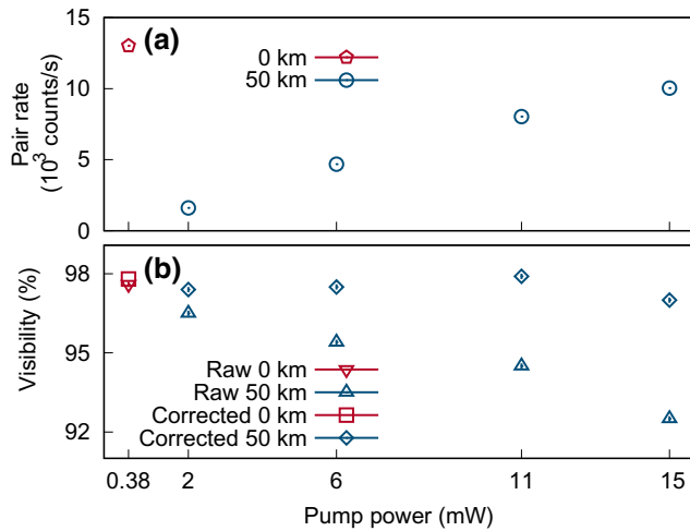
FIG. 3. (a) Average pair rates for different pump powers. The locally collected photon pair rate, averaged over H/V and D/A bases, is 13\,012 \pm 14\text{ s}^{-1} at 380\text{ }\mu\text{W} pump power. Pair rates with the 50-km fiber in the signal arm are 1606 \pm 3\text{ s}^{-1} , 4686 \pm 6\text{ s}^{-1} , 8033 \pm 10\text{ s}^{-1} , and 10\,033 \pm 16\text{ s}^{-1} at their corresponding pump powers. (b) Visibility of polarization correlations as a measure of entanglement quality for different pump powers. The raw visibility observed locally with 380\text{ }\mu\text{W} pump is 97.6 \pm 0.1\% . After propagating through 50 km of SMF28e+ fiber, the raw visibility reduces to 96.5 \pm 0.1\% , 95.4 \pm 0.1\% , 94.5 \pm 0.1\% , and 92.5 \pm 0.1\% for a respective pump power of 2, 6, 11, and 15 mW. Background-corrected visibilities range from 97% to 98% for all the measurements.
