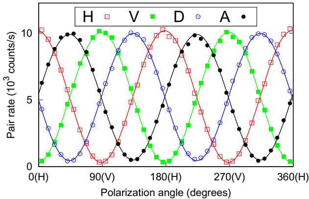
FIG. 4. Polarization correlations in both H/V and D/A bases measured at 15-mW pump power after transmission of the signal photons through 50 km of SMF28e+ fiber. The coincidence rate is measured with polarization optics before signal and idler photon detection, as shown in Fig. 1. The polarization on the idler side is kept at one of the four linear settings (H, V, D, and A) whereas the polarization on signal side is rotated over 360^\circ using the half-wave plate.
