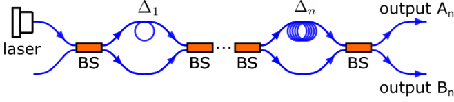
FIG. 3. Scheme to efficiently generate thermal photon-bunched light from coherent laser light by using a cascaded series of asymmetric Mach-Zehnder fiber interferometers. The input field is first split by a beamsplitter (BS), with one arm acquiring a propagation delay \Delta_1 before recombination at a subsequent beamsplitter with the non-delayed arm. The interferometric loop can be repeated n times, with each stage introducing progressively longer fiber delays \Delta_n , providing two single-mode outputs ( A_n, B_n ).
